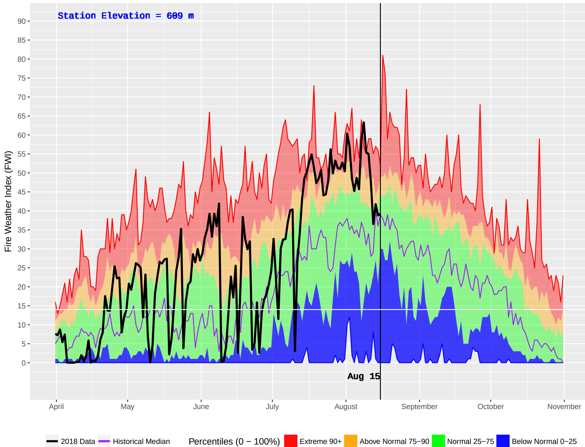
ROCK CREEK (394) : Historical (1990–2016) and Current (2018) Daily Fire Weather Index (FWI)
