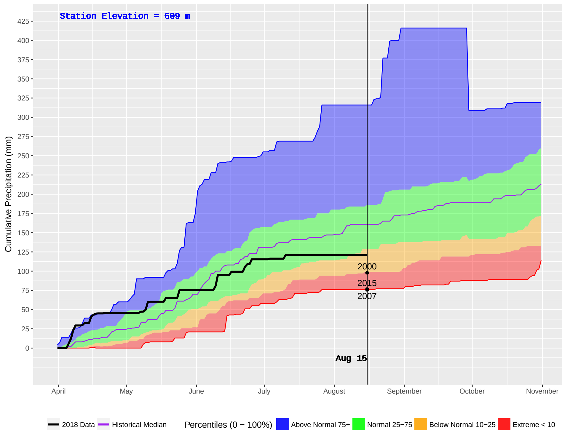
ROCK CREEK (394) : Historical (1990–2016) and Current (2018) Daily Cumulative Precipitation
